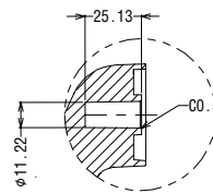
DETAIL B SCALE 2:1
